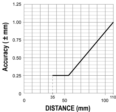
Figure 24. 110 mm Models
