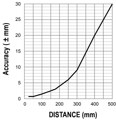
Figure 15. 500 mm Models
